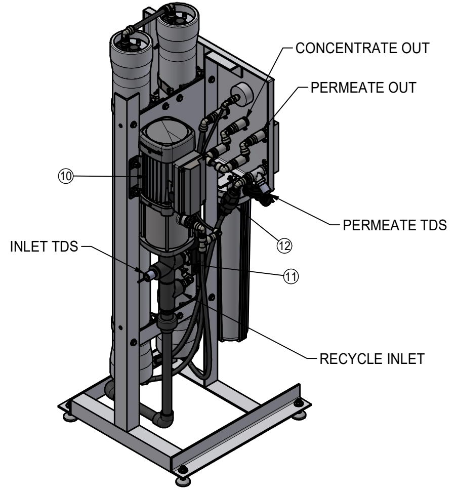
ISOMETRIC VIEW
