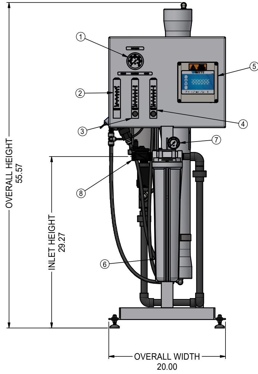
FRONT VIEW
