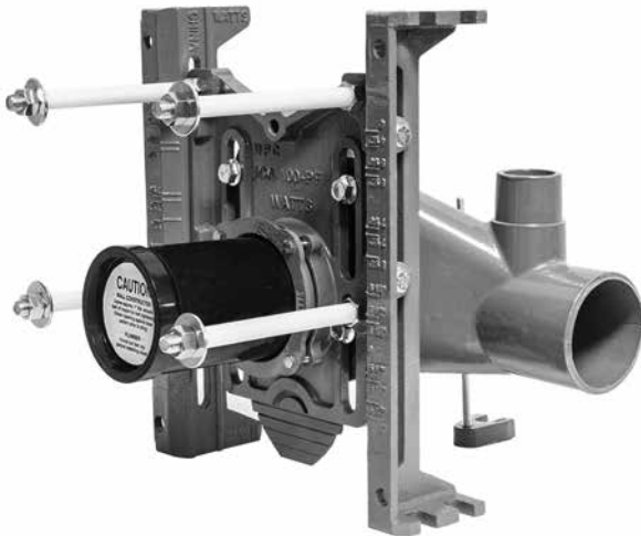
Industry Standard Compression Seal Carrier
